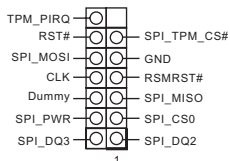
SPI_TPM_J1
