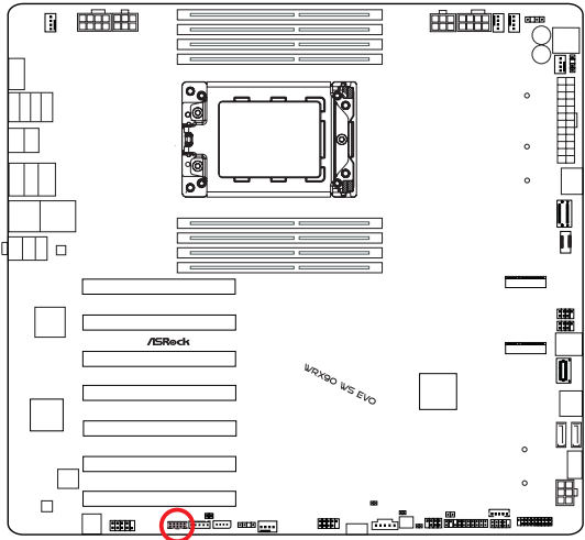
VGA_CON1
