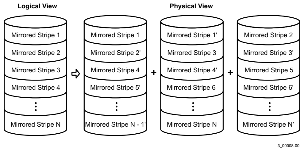
Figure 3 Integrated Mirroring Enhanced with Three Disks
