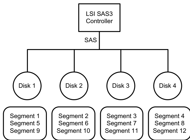
Figure 8 Integrated Striping Example
