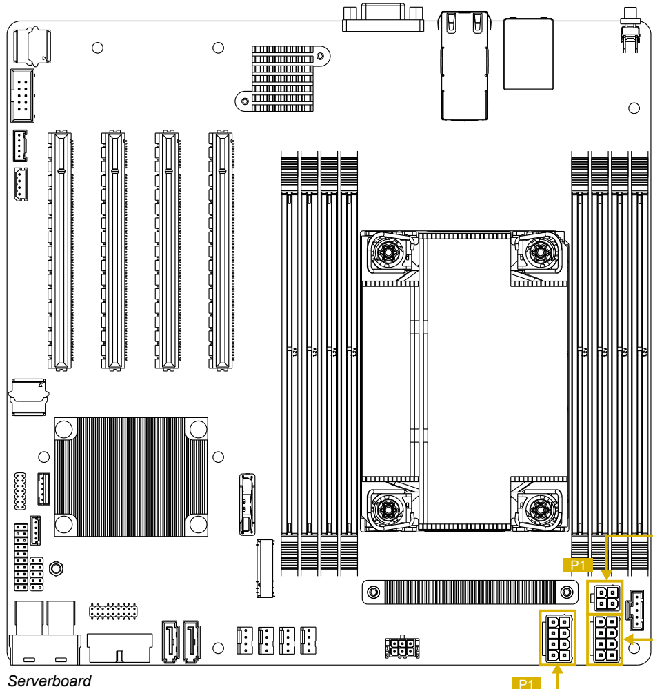
Serverboard
