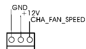
39 : 3-Pin Chassis FAN Connector (+12V)
