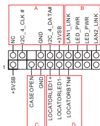
Auxiliary Panel Header (18-pin AUX_PANEL1) (see p.22, 25, 28, 31)
