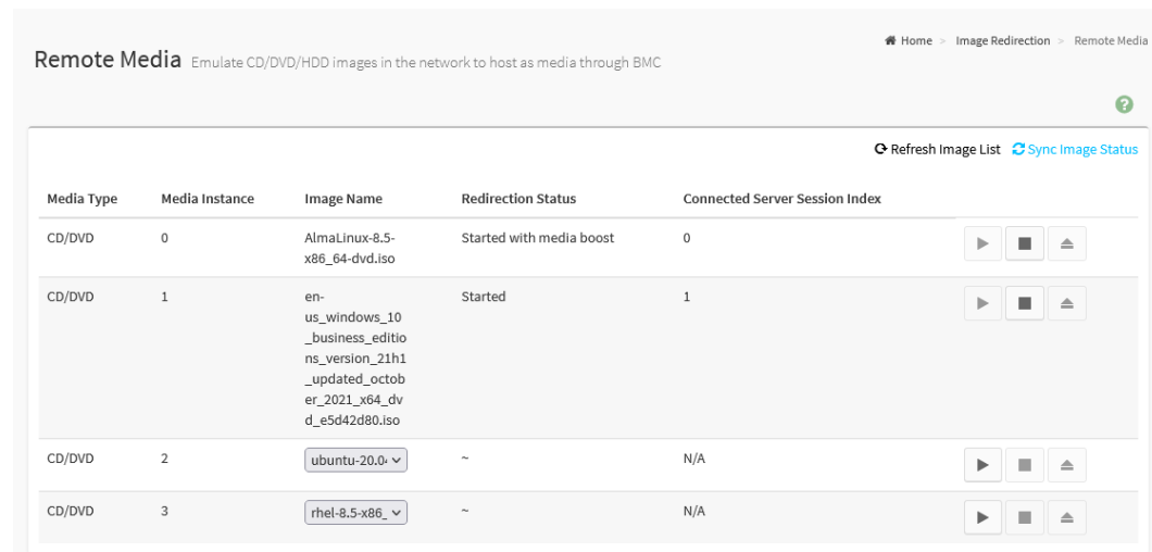
Figure 116. Snapshot of Remote Images Page
