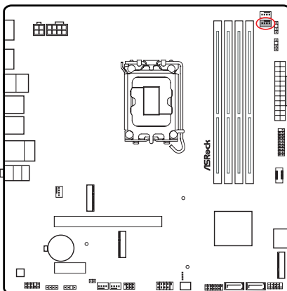
CPU_FAN2/WP
