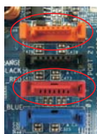
SATAII_RED (PORT1) and SATAII_ORANGE (PORT3)
