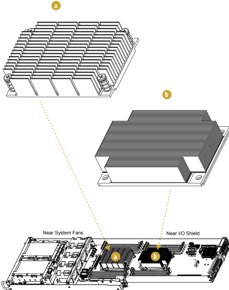
Heatsink Type
