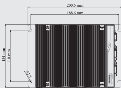
Dimension of the iEP-7040E-020, iEP-7041E-020, iEP-7040E-025, iEP-7041E-025 with Wall Mounting Bracket Installed
